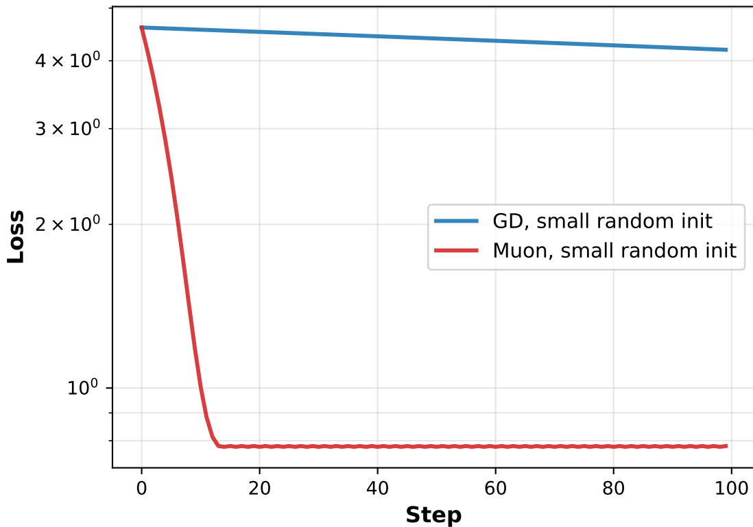
Loss: GD vs Muon (small random init)
